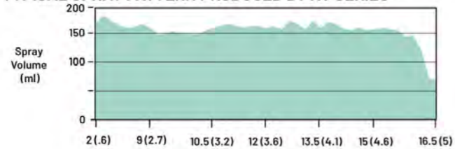
TYPICAL SPRAY PATTERN PRODUCED BY XT SERIES
